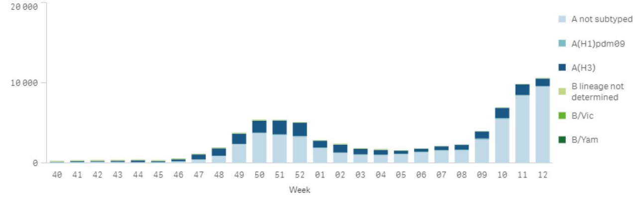
Influenza virus detections by type, subtype/lineage and week - WHO Europe, season 2021/2022
